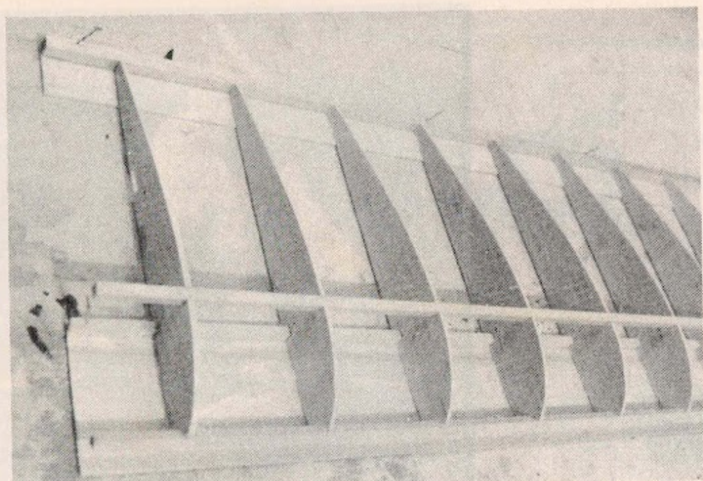
The top wing assembly is begun.
