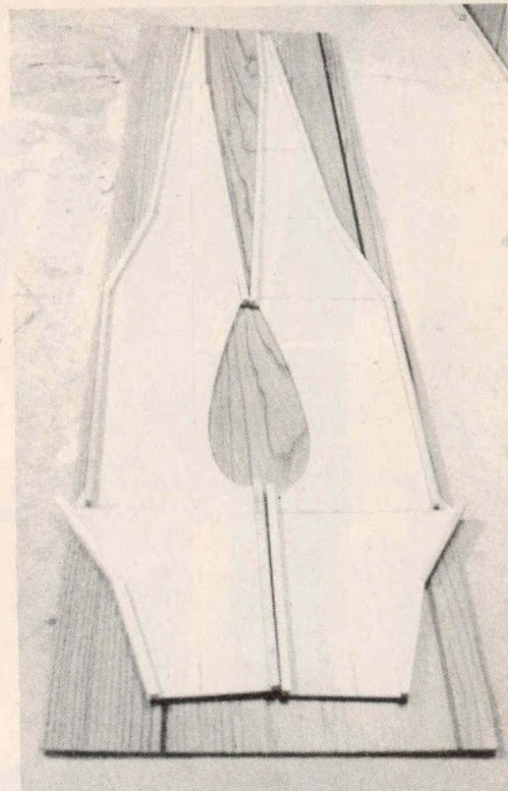
The fuselage sides with longerons glued in place.
