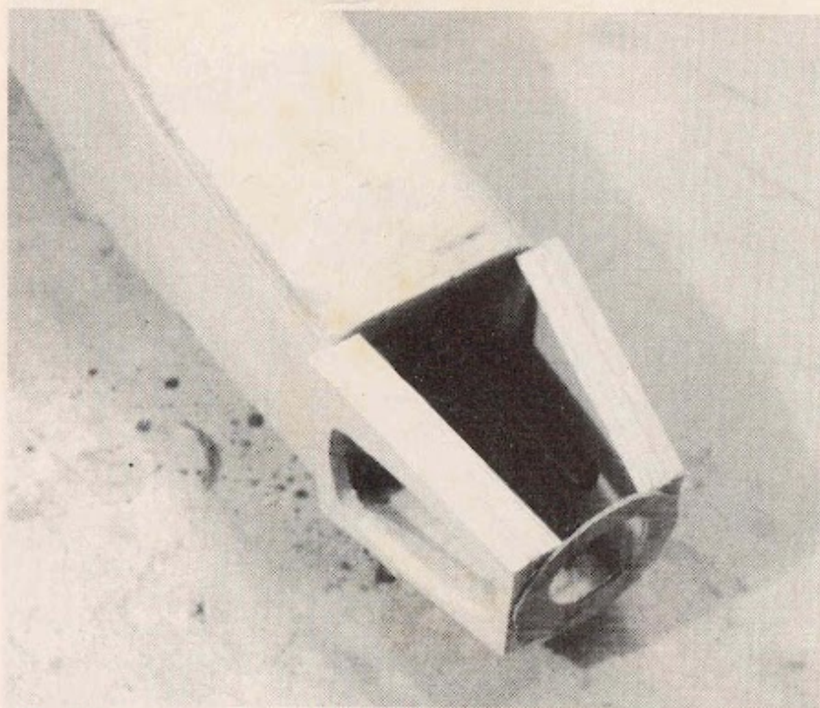
The balsa nose (cowl) is built up from balsa sheet and triangular stock.
