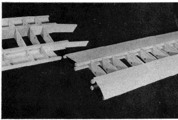
Top sheeting was installed while wing panels were flat on building board.
